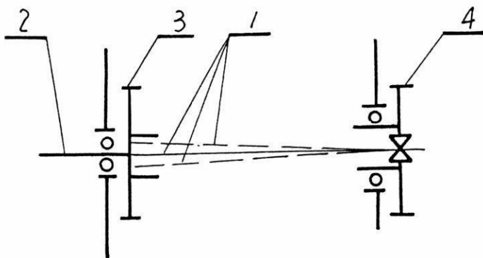
1 main shaft 2 input shaft 3 input shaft gear 4 gear box drive gear figure 2-5 gear box two shaft floating structure
