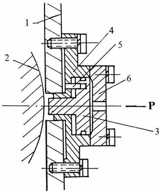
2. 1. Gear box shell counter shaft gear 3. Clutch brake cylinder piston. The clutch brake cylinder 5. Guide pin 6. Side cover figure 2-8 clutch brake cylinder
